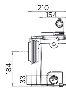
Dimensions (mm)
